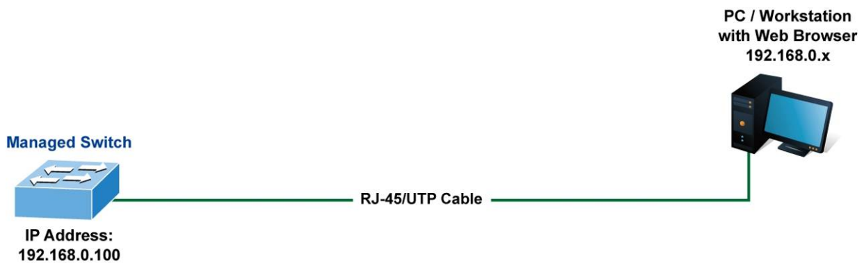
Figure 4-1-1: Web Management
