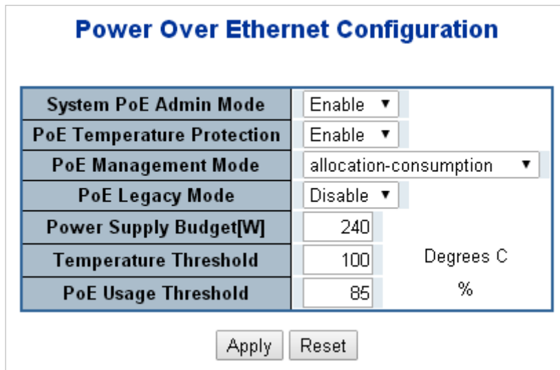
Figure 4-16-2: PoE Configuration Screenshot
