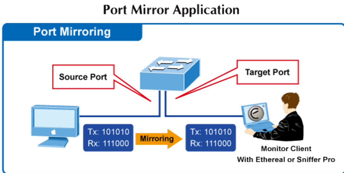
Figure 4-4-5: Port Mirror Application
